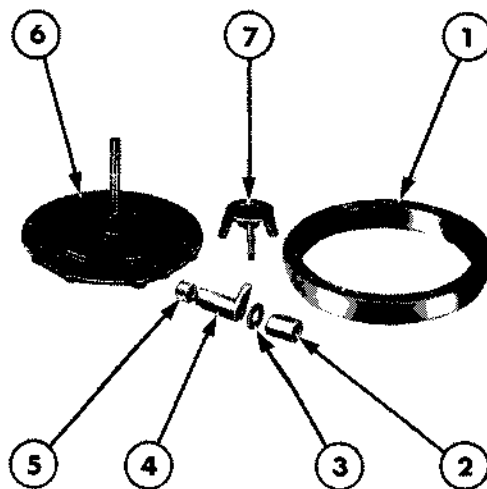
Figure 19 TW-15, TW-25 and TW-35 Clutch Tools 1. Adaptor Ring, Tool No. 1194 2. Spindle Nut, Tool No. 1280 (SW 510-9) 3. Thrust Washer, Tool No. 1281 (SW 510-10) 4. Release Lever Gauge, Tool No. 1267 (SW 510-2) 5. Gauge Spacer, Tool No. 1193 6. Fixture Base, Tool No. 1283 (SW 510-60) 7. Bridge, Tool No. 1268 (SW 510-3)
